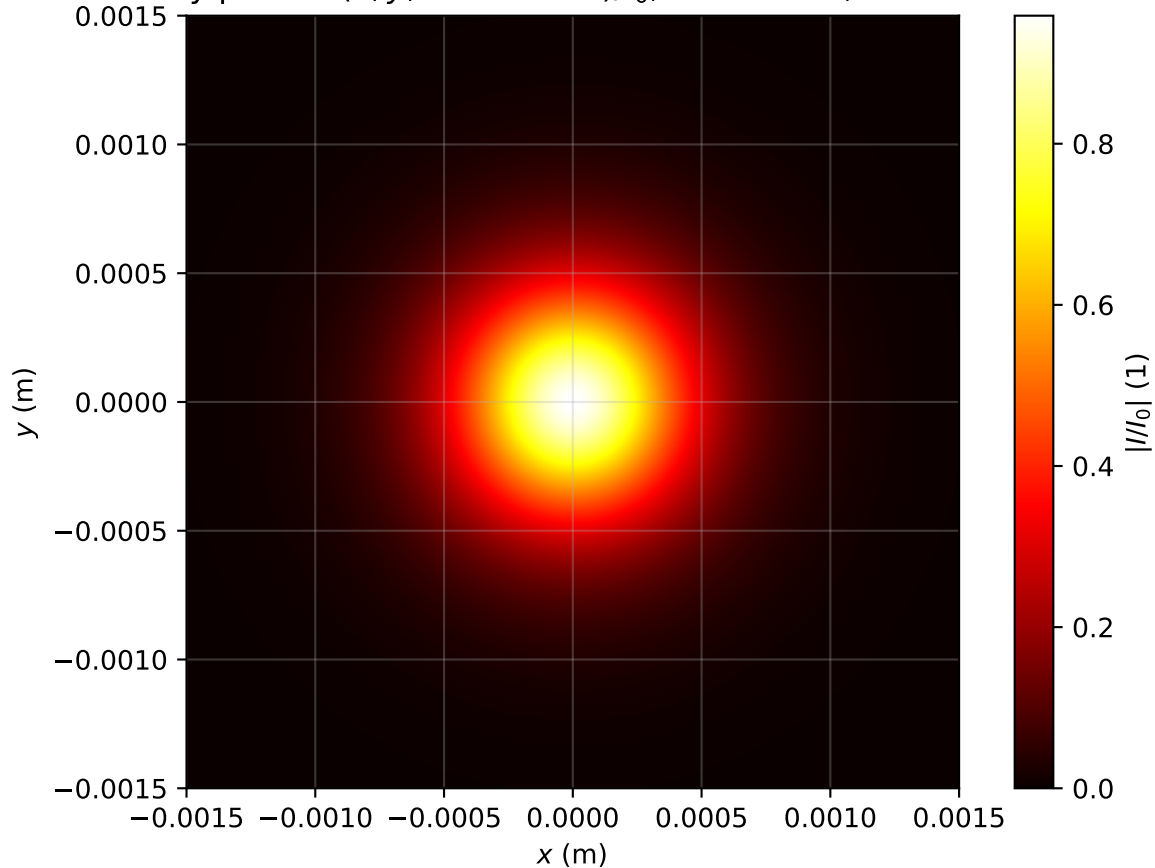
Intensity profile I(x, y, z = 2.548m)/I_0 , P_{in}=0.7P_{cr} , artificial time
